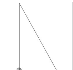
geometric right triangle
