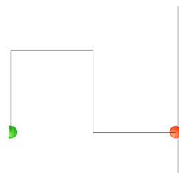
geometric checker board
